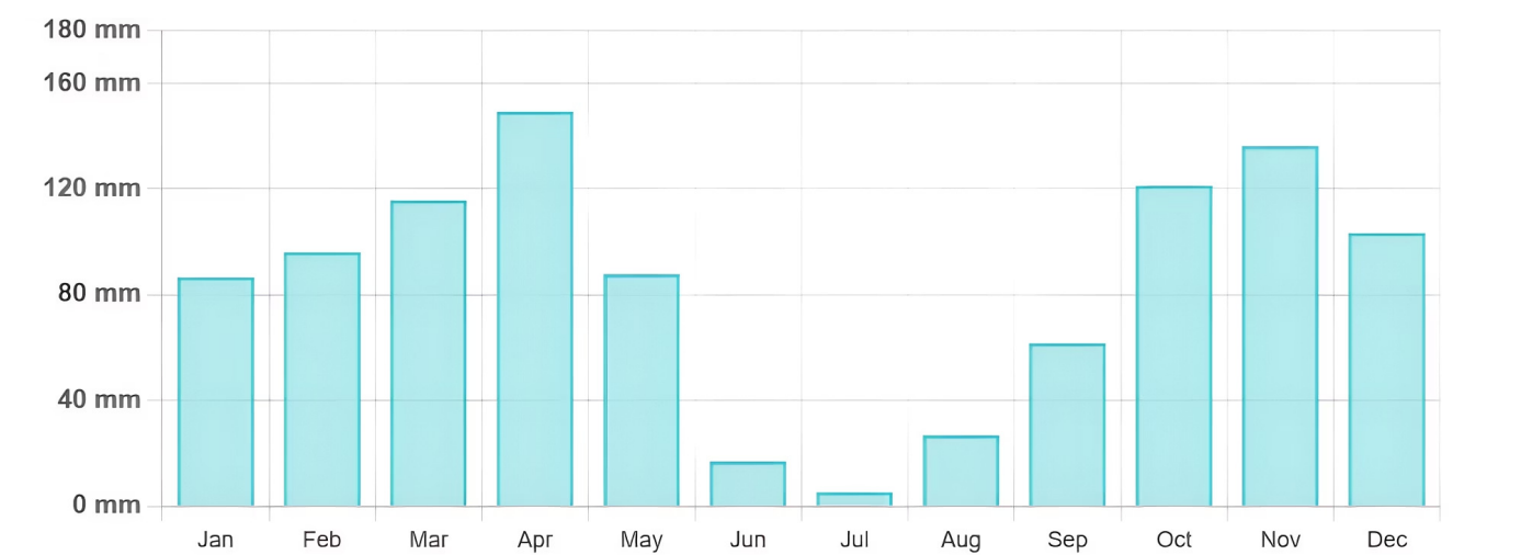
Figure 3: Rainfall variability on a monthly basis
